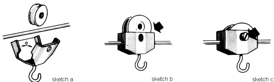
Fig. 6: Assembly of the cable trolleys
