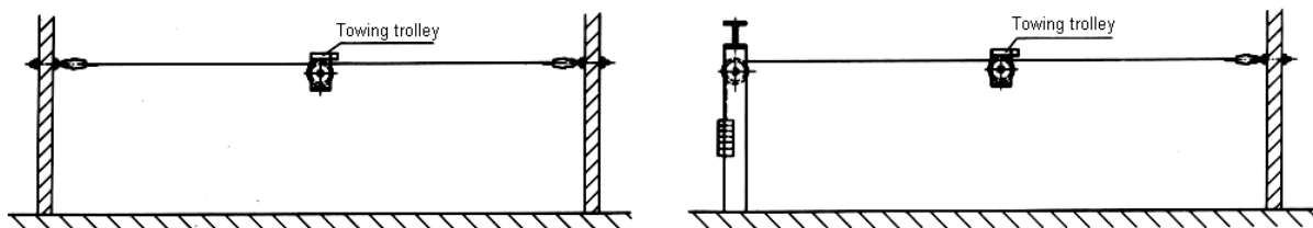
Fig. 3: Types of arrangement for the rope fixation
